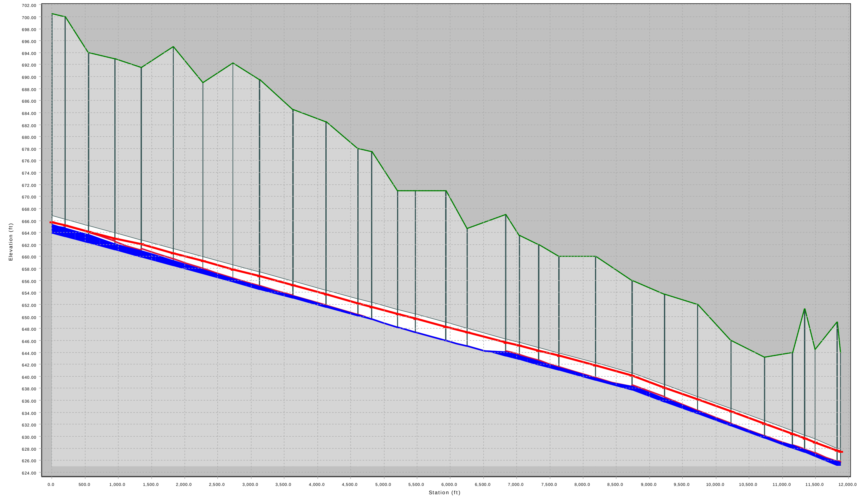
Future Design Peak Flow Conditions (July 6 Event) without Sluice Gate and Pumping Station Route A 36-Inch Pipe
