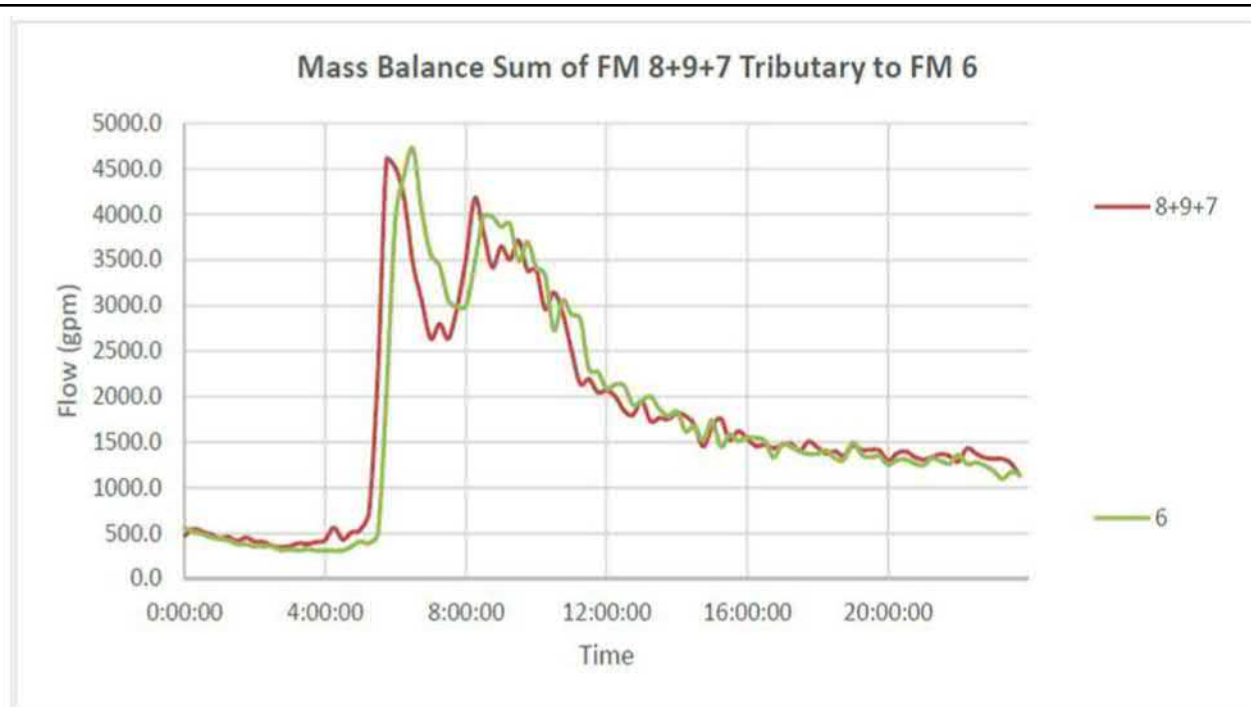
Figure 2.02-7 Mass Balance at FM-6–July 6, 2016, Wet Weather Conditions
