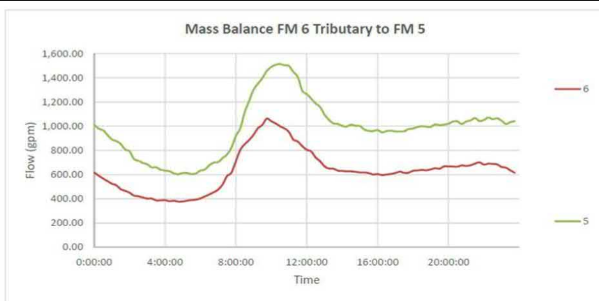
Figure 2.02-4 Mass Balance at FM-5–Dry Weather Conditions
