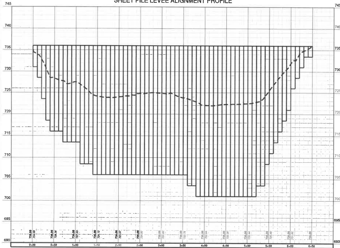
SHEET PILE LEVEE ALIGNMENT PROFILE
