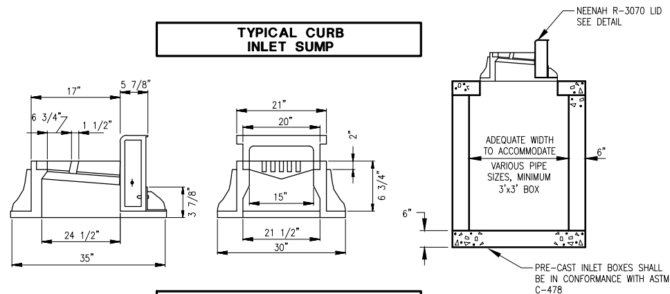
CURB INLET
