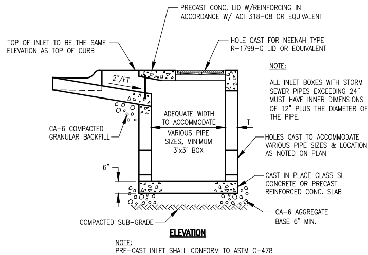
OPEN THROAT INLET
