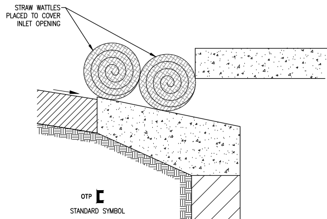
OPEN THROAT INLET SEDIMENT PROTECTION - STRAW WATTLES
