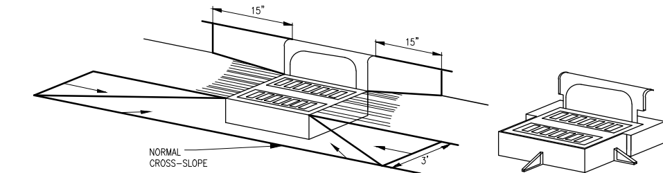
TYPICAL CURB INLET SUMP
