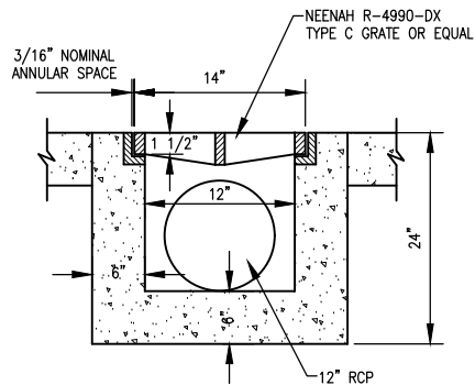
TRENCH DRAIN
